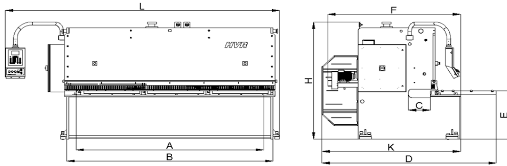
CNC-HVR HYDRAULIC VARIABLE RAKE GUILLOTINE SHEAR SPECIFICATIONS
